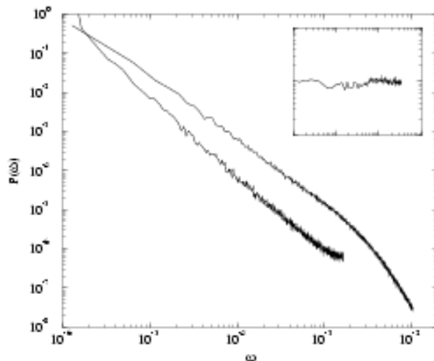
Fig. 5. — Fourier transform of the price autocorrelation function \langle x(t)x(t+\tau) \rangle as a function of temporal frequency for the DEM-USD exchange rate (Oct 1991-Nov 1994) ( bottom curve ) as compared to the k^{-5/3} power-law spectrum observed for the spatial velocity fluctuations in turbulent flows (the data were recorded by Y. Gagne and collaborators in a wind tunnel experiment at R_\lambda = 3050 ) ( top curve ). Inset: Fourier transform of the price change autocorrelation function \langle \Delta x(t)\Delta x(t+\tau) \rangle , which is completely flat (and would behave as the 1/3 - th power of frequency in turbulent flows). Units are arbitrary.
