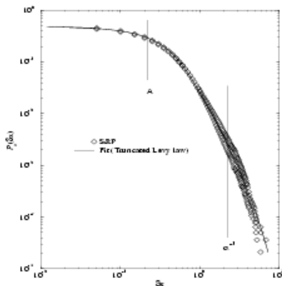
Fig. 3. — Rank ordering of 5-minute increments of S&P 500 index futures. The cumulative distribution function of price increments is well represented by an exponentially truncated Lévy distribution with finite variance.
